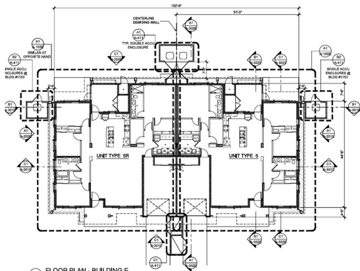
B1 FLOOR PLAN - BUILDING E SCALE: 1/8"=1'-0"
