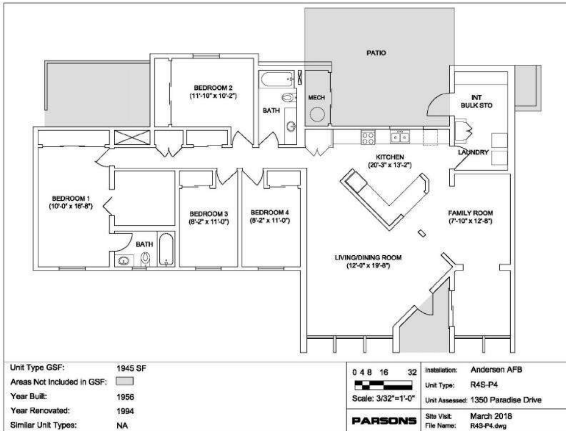
FIELD GRADE OFFICER 4 BEDROOM - R4S4
