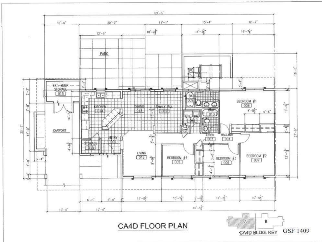
JUNIOR ENLISTED 4 BEDROOM - CA4D11/CA4D12
