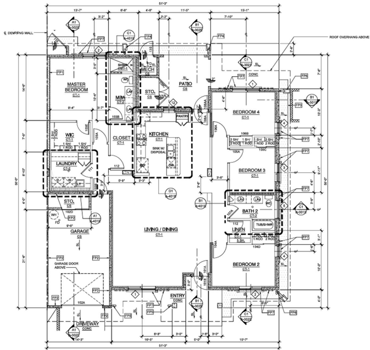
A1 FLOOR PLAN - UNIT TYPE 5 SCALE: 1/4"=1'-0" (NOTE: UNIT TYPE SR SIMILAR AT OPPOSITE HAND)
